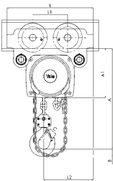
Model Yalelift ITP ATEX, 500 - 3000 kg, single fall
