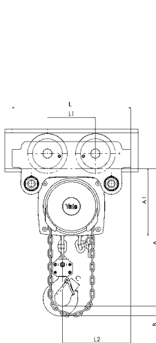
Model Yalelift ITP ATEX, 500 - 3000 kg, single fall
