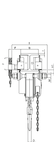
Model Yalelift ITP ATEX, 500 - 3000 kg, single fall
